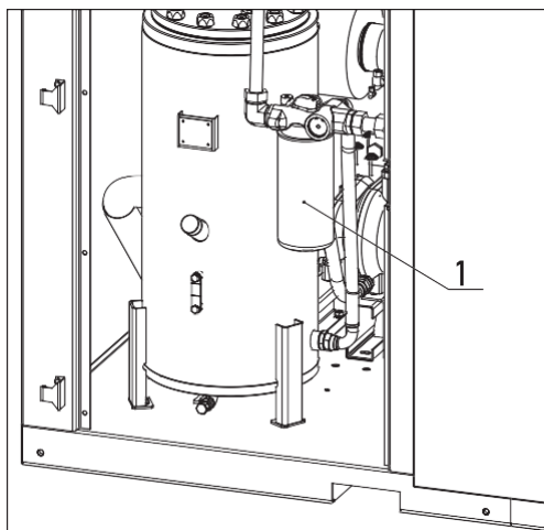
Fig. 5.3.2 Oil Filter replacing
