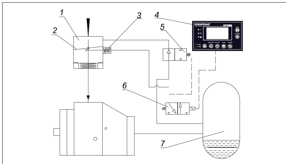
Fig. 2.5 Control system
